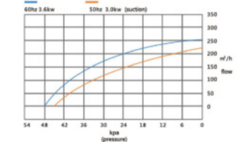
GB series vortex air pump performance curve (for reference only, do not take it for testing standard)
