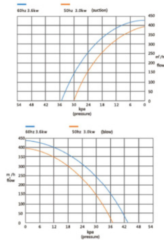
GB series vortex air pump performance curve (for reference only, do not take it for testing standard)
