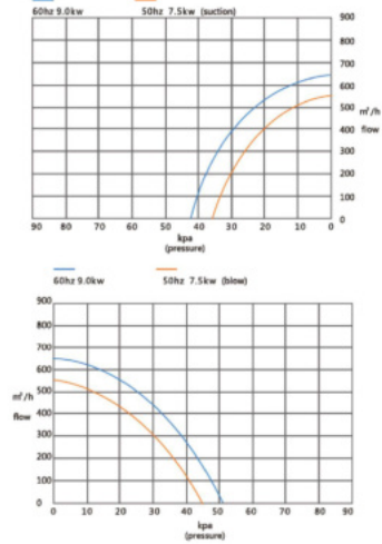
GB series vortex air pump performance curve (for reference only, do not take it for testing standard)
